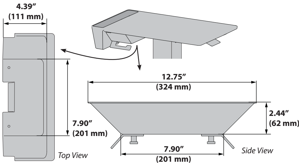
Side View
